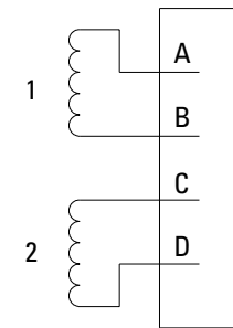
Solenoid Valve Schematic
