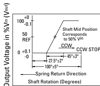
Potentiometer Output Characteristics (Output Voltage Versus Shaft Rotation)
